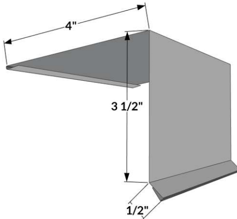
HE-2 - High Eave Trim
