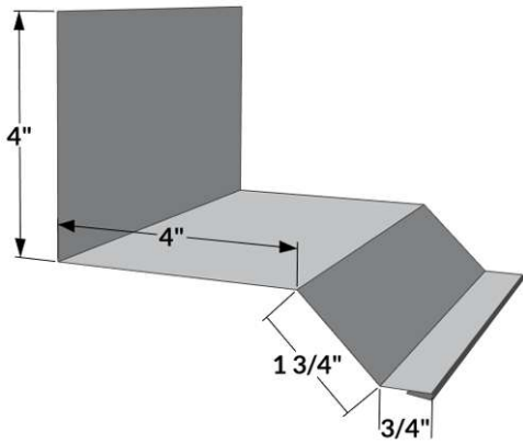
RTW-21 Roof to Sidewall (1236)
