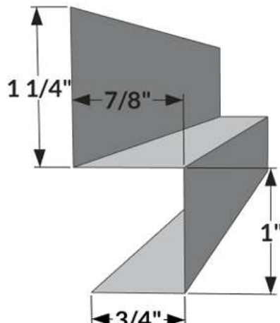
BT-2 - Base Trim
