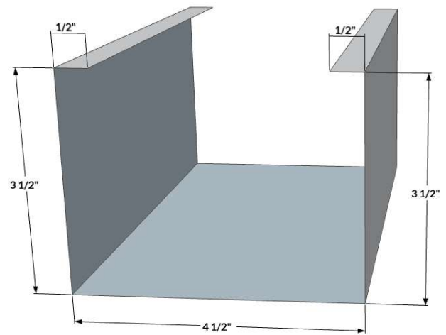
DS-1 - Downspout
