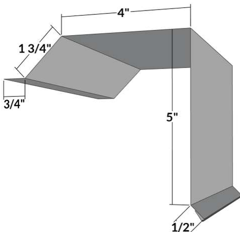
GT-41 - Gable Trim (1236)
