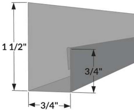
JT-1 - J Trim (Siding)
