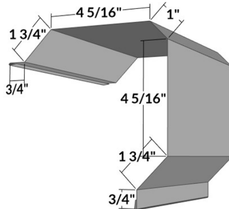
OC-4 - Outside corner 1236
