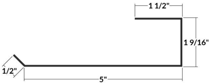
GT-7P1 - 2 pc Gable trim Base Pan
