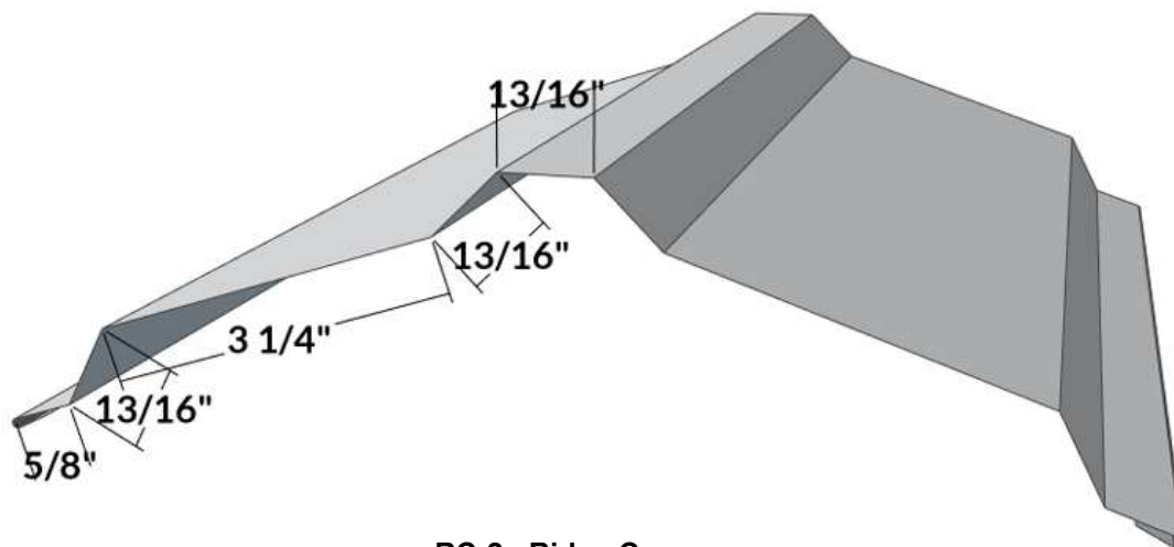
RC-2 - Ridge Cap
