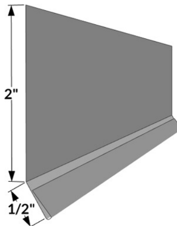
SDS-1 - Siding Starter
