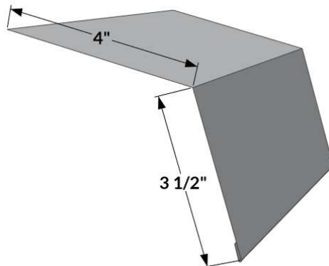
26-ET-WG - Roof Eave Trim
