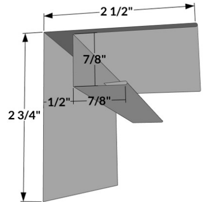
SST-1 - Soffit Starter
