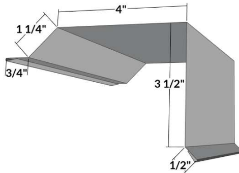
GT-2 - Gable Trim (936)
