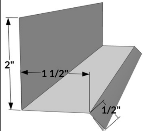
DC-3 Drip Cap
