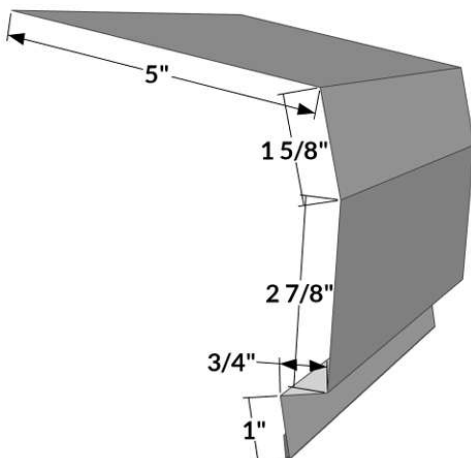
26-ET-NG - Roof Eave Trim
