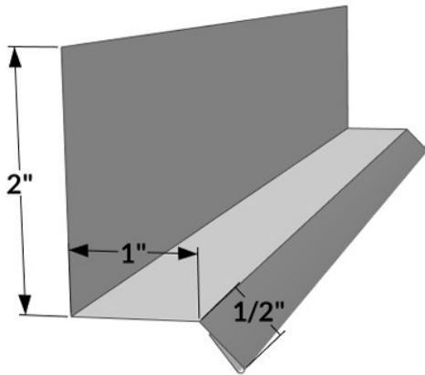
DC-1 - Drip Cap
