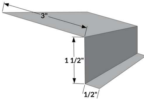
RE-1 - Roof Eave Trim (no gutter)
