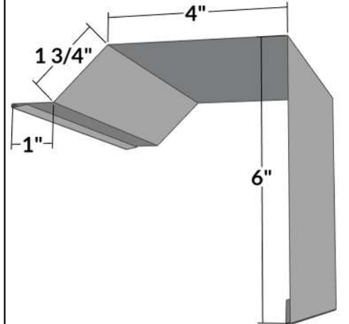
GT-31 - Gable trim (1236)
