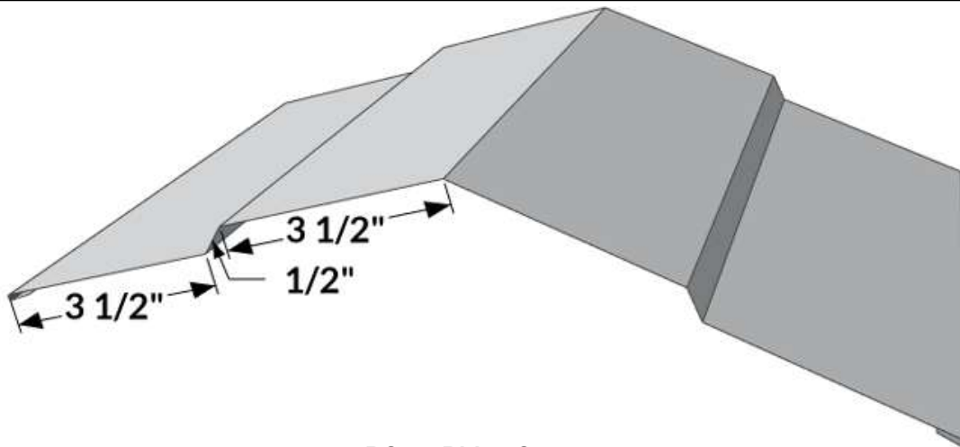
RC-4 - Ridge Cap
