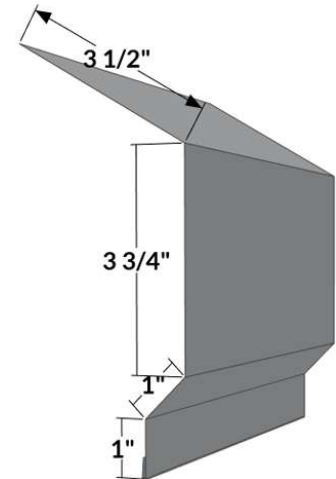
ET-2 - Roof Eave Trim
