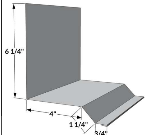
RTW-3 - Roof to Sidewall (936)
