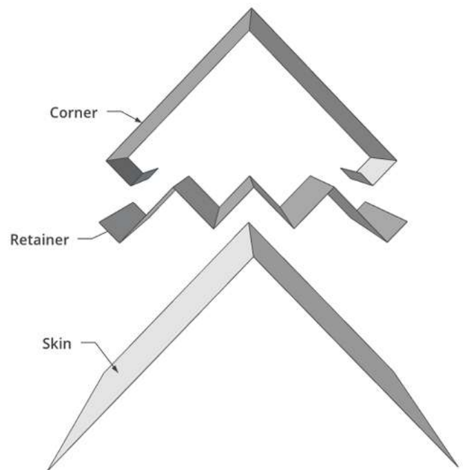
OC-4 - Outside corner 1236
