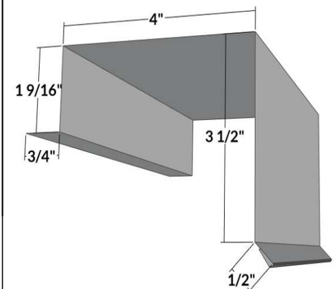
GT-6 - Gable Trim (Snaplock/SSR)
