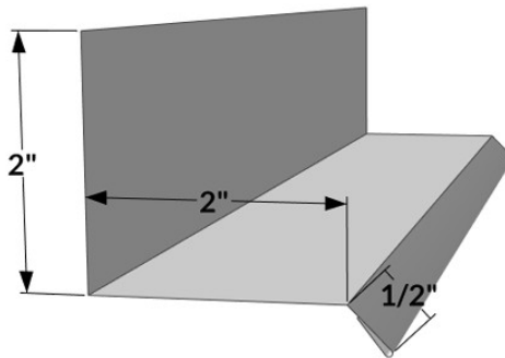
DC-5 - Drip Cap
