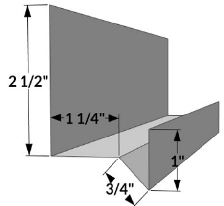
DWC-1 - Drip Cap
