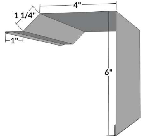
GT-3 - Gable Trim (936)
