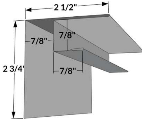
ILC-2 - Inside Corner
