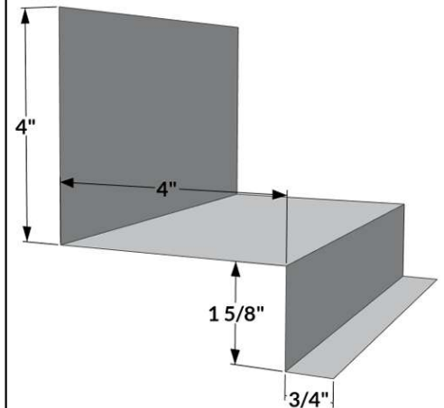
RTW-4 - Roof to Sidewall Snaplock/SSR
