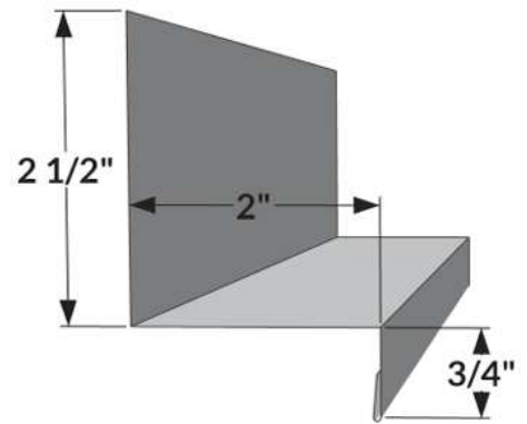
BF-3 - Base Flashing
