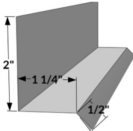
DC-2 - Drip Cap
