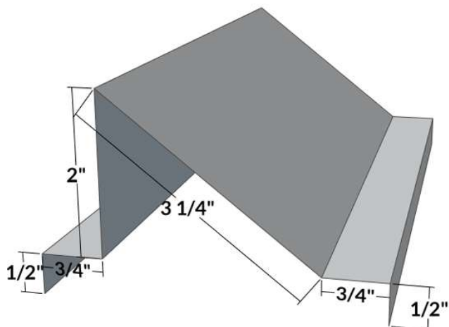
SS-2 - 2pc Snow Stop (SSR)
