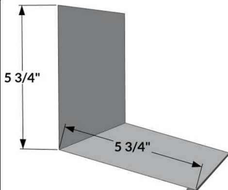
RTW-1 - Roof to High Wall
