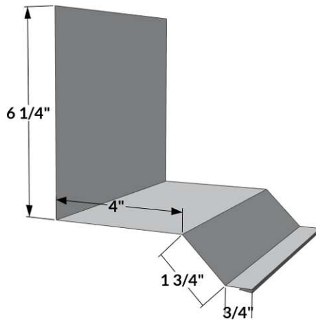
RTW-31 - Roof to Sidewall (1236)
