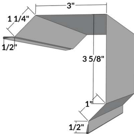
GT-1 - Gable Trim (936)
