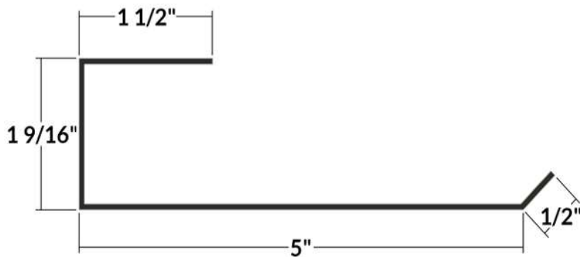
RTW-5P1 - 2pc Roof to Sidewall Base Pan
