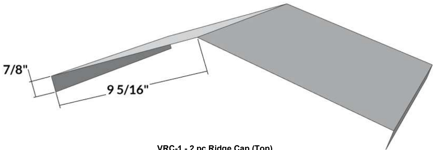
VRC-1 - 2 pc Ridge Cap (Top) SSR/Snaplock
