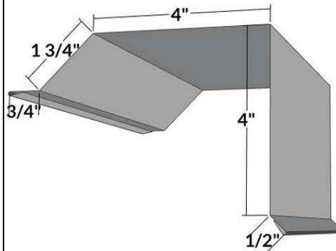
GT-21 - Gable Trim (1236)
