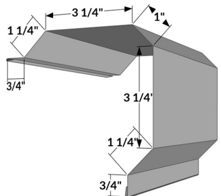
OC-3 Outside corner 936
