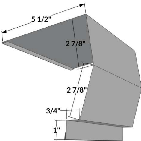
HE-1 - High Eave trim
