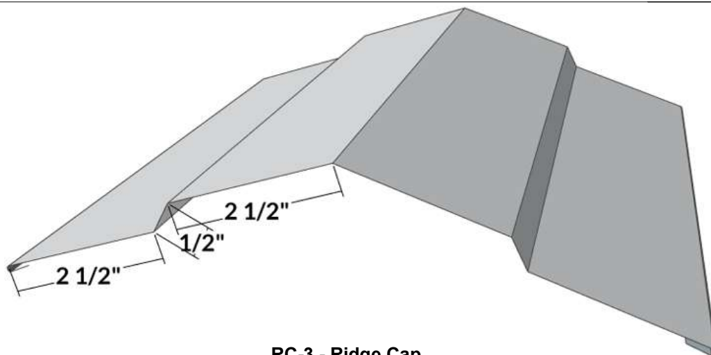
RC-3 - Ridge Cap
