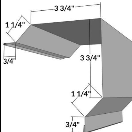
OC-2 - Outside Corner 936
