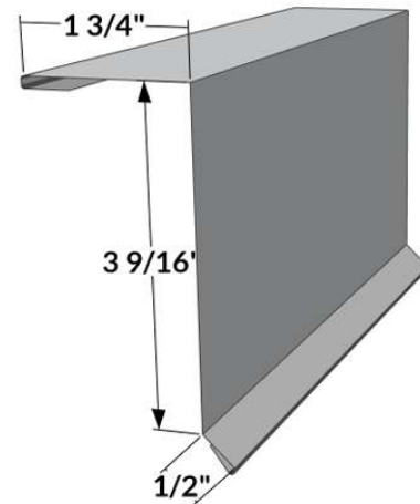
GT-7P2 - 2 pc Gable trim Top
