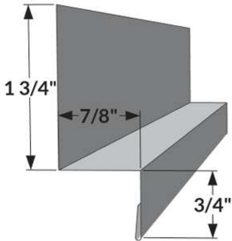
BF-1 - Base Flashing
