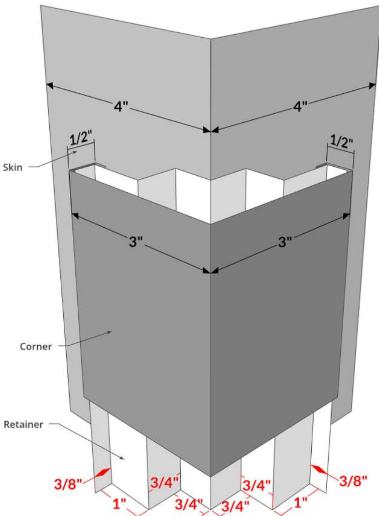
OC-21 - Outside Corner 1236
