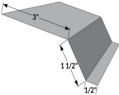
RF-1 - Roof Eave trim (for gutter)
