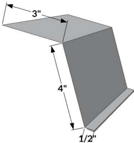
ET-1 - Roof Eave Trim
