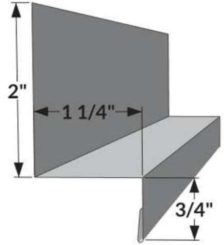
BF-3 - Base Flashing
