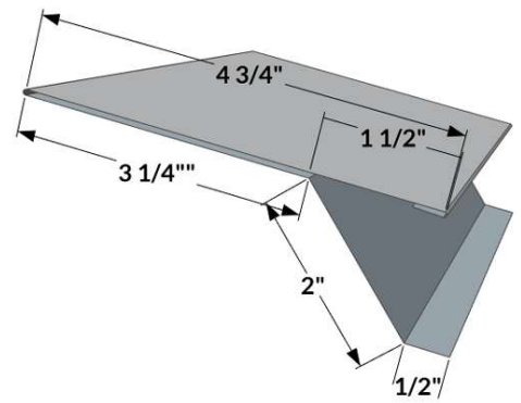
RFH-1 - Eave Trim for Snaplock/SSR
