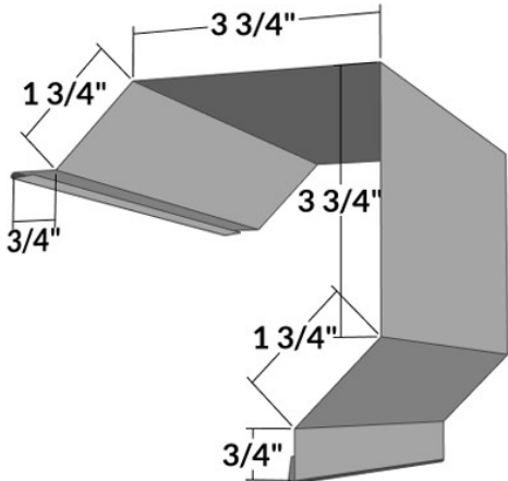
OC-21 - Outside Corner 1236
