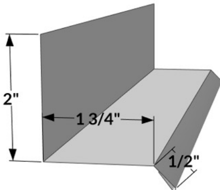
DC-4 - Drip Cap
