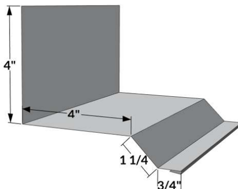
RTW-2 - Roof to Side Wall (936)
