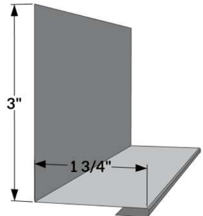
RTW-5P2 - 2pc Roof to Sidewall Top
