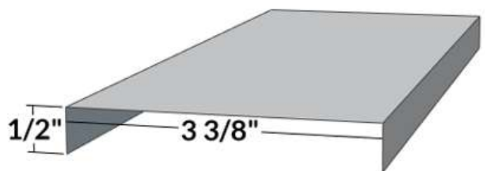
SS-2C - Snow Stop Channel (SSR)
