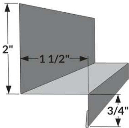
BF-4 - Base Flashing
