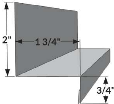
BF-2 - Base Flashing
