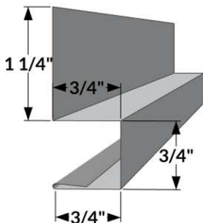
BT-1 - Base Trim (Siding)
