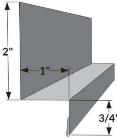
BF-2 - Base Flashing
