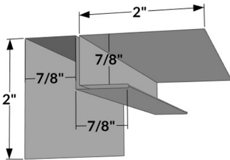
ILC-1 - Inside Corner (29 ga only)
