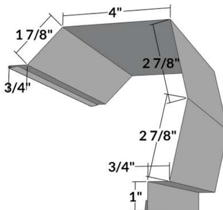
GT-5 - Gable Trim (1236)
