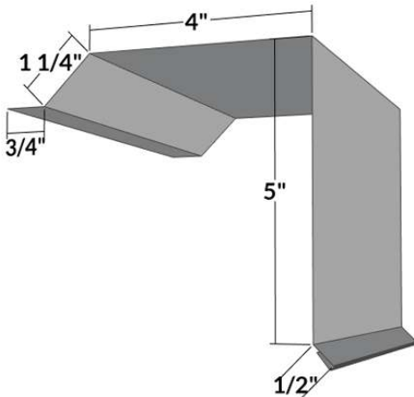
GT-4 - Gable Trim (936)
