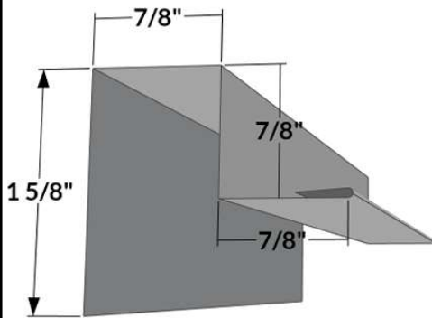
WC-1 - Wall to Ceiling
