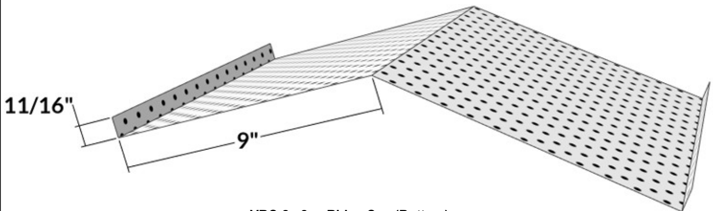
VRC-2 - 2pc Ridge Cap (Bottom) Perforated and Non-Perf SSR/Snaplock
