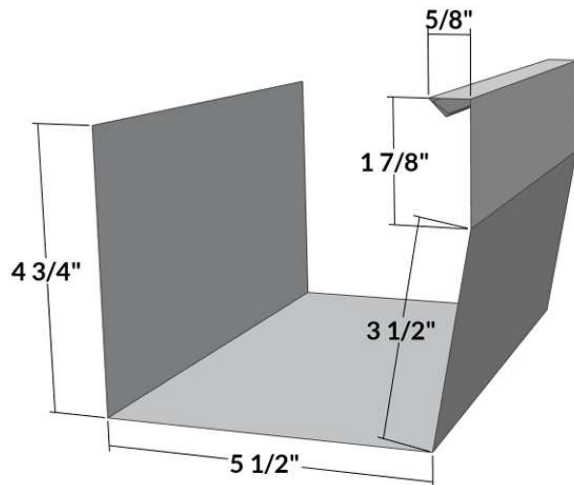
EG-2 - Gutter
