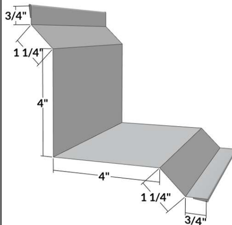
IC-1 - Inside Corner 936
