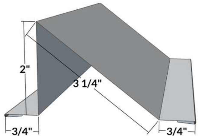
SS-1 - Snow stop
