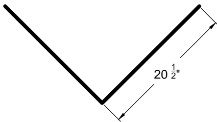
VALLEY FLASHING VF-1
