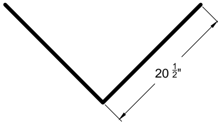
VALLEY FLASHING VF-1
