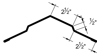
DELUXE RIDGE CAP RC-3
