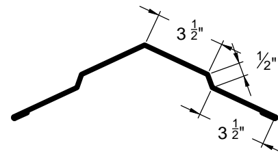
DELUXE RIDGE CAP RC-3 7.75
