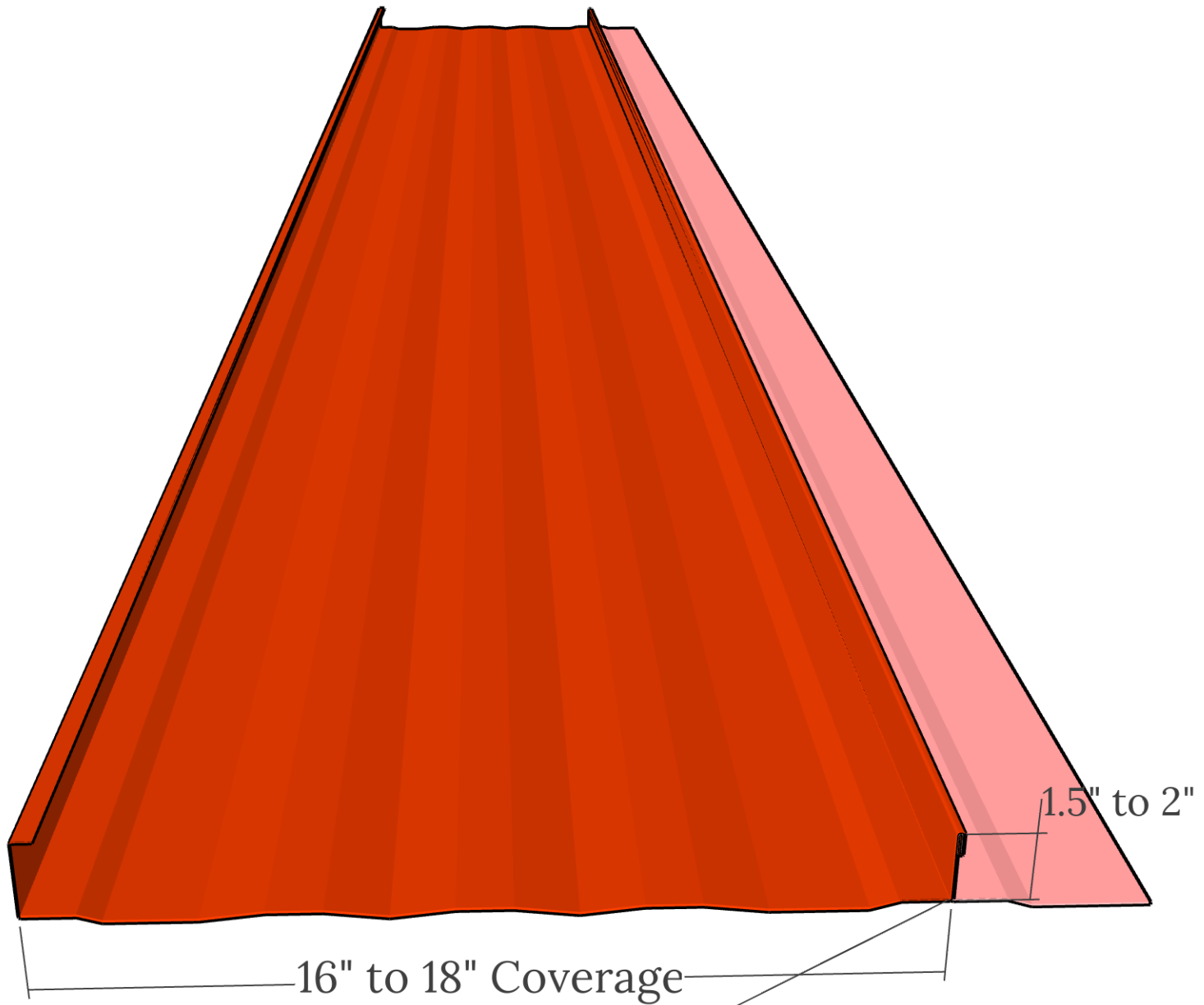
SSR150 and SSR200 Standing Seam Roof Profile
