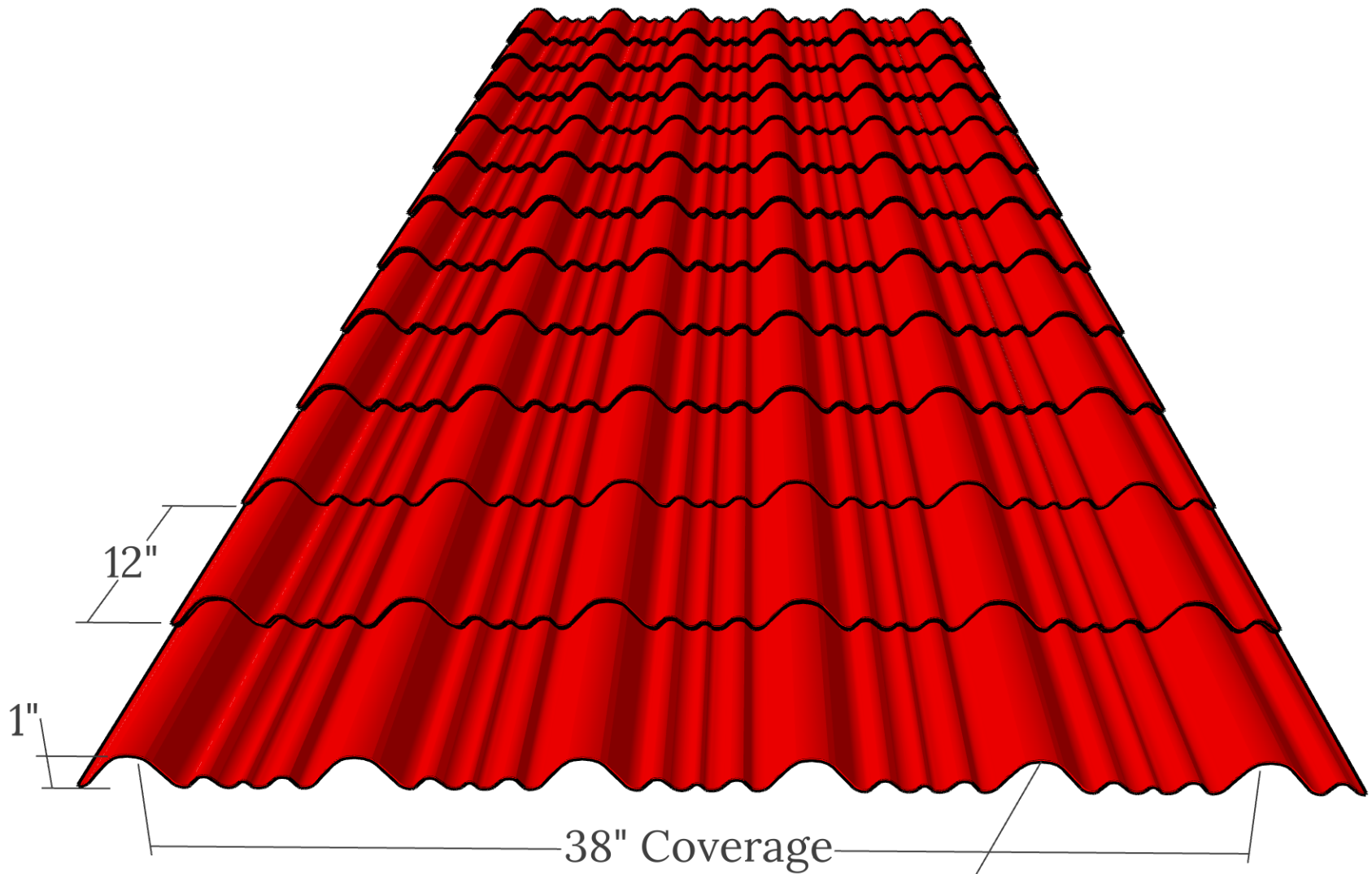
838T Stamped Roof Profile
