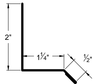
DRIP CAP DC-2
