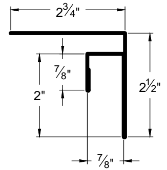
SOFFIT STARTER ST-1
