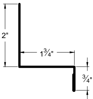
BASE FLASHING BF-5
