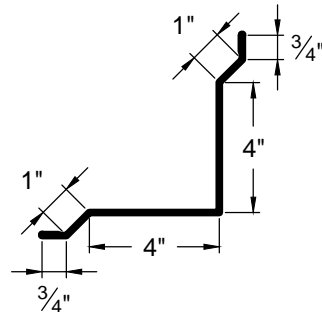
INSIDE CORNER IC-1
