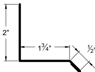
DRIP CAP DC-4
