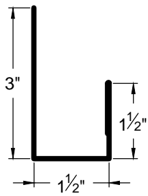
J TRIM JT-4
