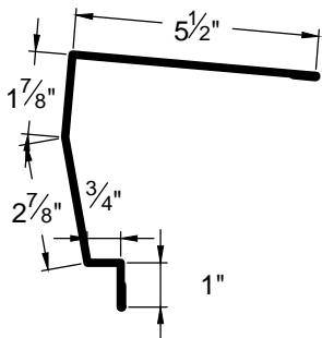
HIGH EAVE HE-1
