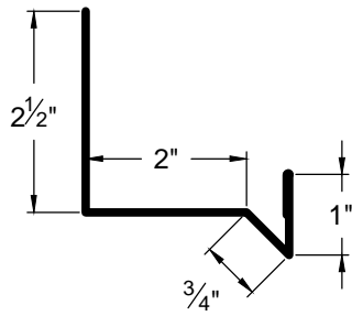
DOOR & WINDOW DRIP CAP RG-1
