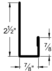
DOWNSPOUT CAP DSC-1
