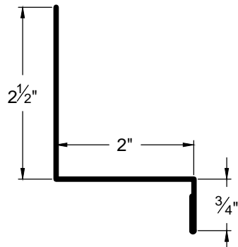
BASE FLASHING BF-6
