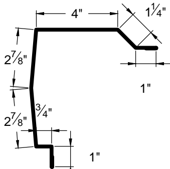
GABLE TRIM GT-5
