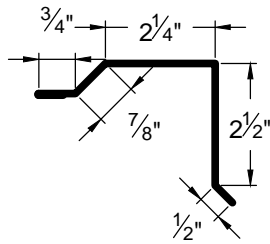
GABLE TRIM GT-2
