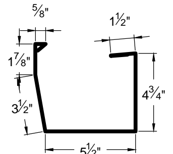
GABLE TRIM GT-4
