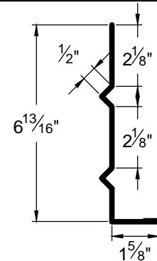
REINFORCED FASCIA REF-1
