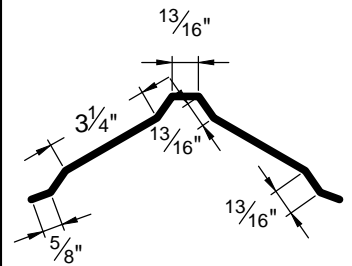
DELUXE RIDGE CAP RC-2
