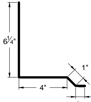
ROOF TO WALL RTW-3
