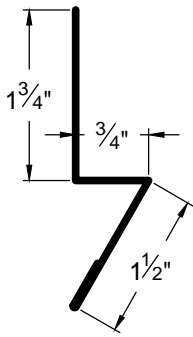
RAT GUARD RG-1
