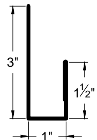
GUTTER EG-2
