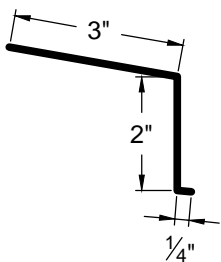
ROOF EDGE RE-1
