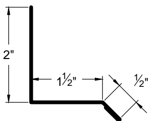
DRIP CAP DC-3
