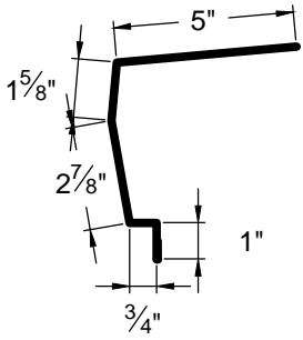
EAVE TRIM (NO GUTTERS) 26-ET-NG
