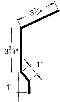
EAVE TRIM ET-2
