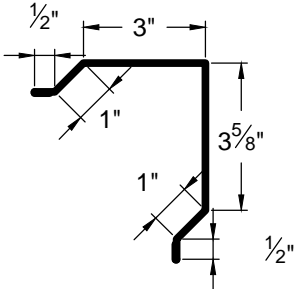
GABLE TRIM GT-1
