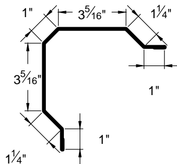
OUTSIDE CORNER OC-3
