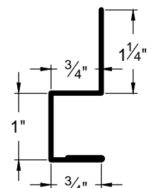
BASE TRIM BT-1
