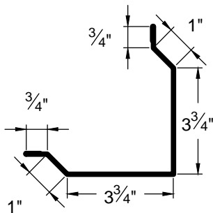
OUTSIDE CORNER OC-2
