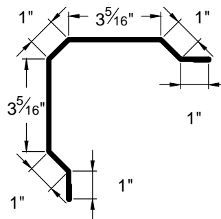
OUTSIDE CORNER OC-4
